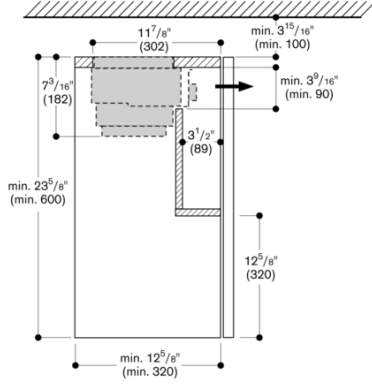
Cross-section of upper cabinet with AA 211 812
