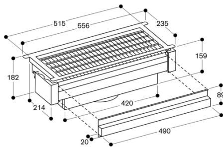
Removable filter panel
