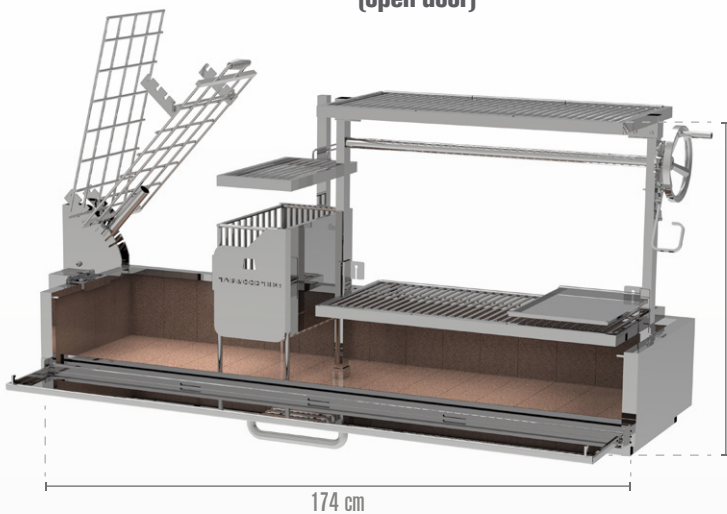
Front view (open door)
